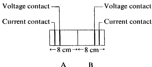
Fig. 1 Configurations for measuring the contact resistivity between old mortar (A) and new mortar (B).
